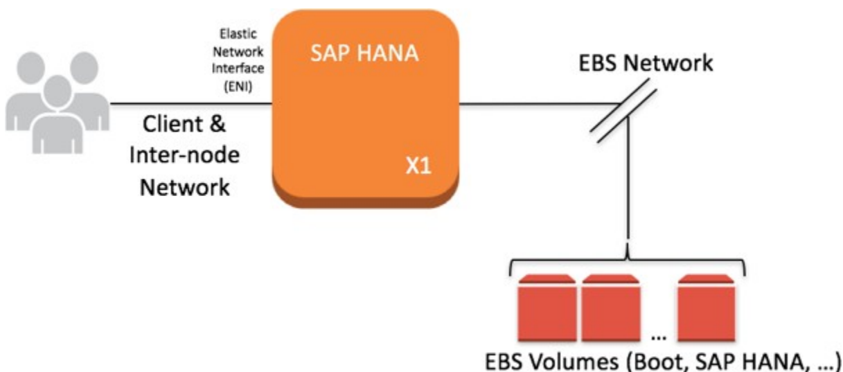
Figure 9: EBS-optimized instances
