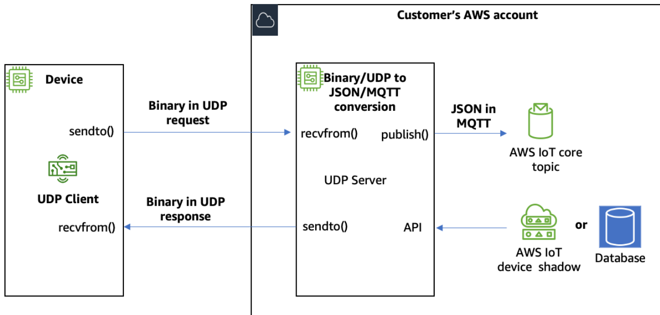
Example architecture for processing UDP datagrams with AWS
