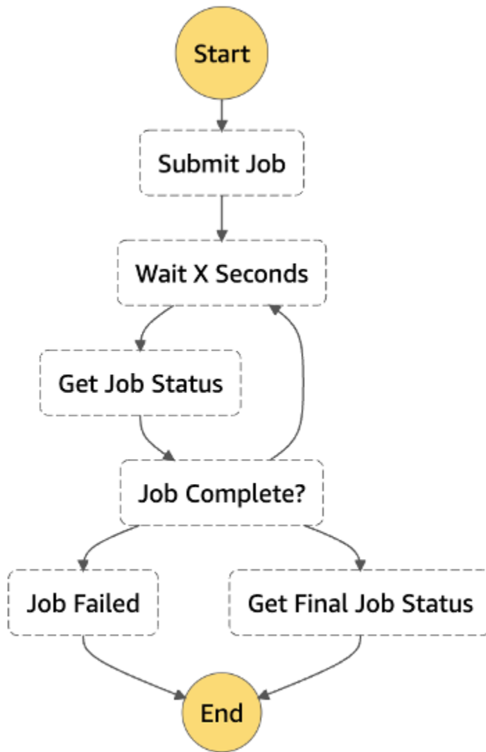
Figure 36: Job Poller
