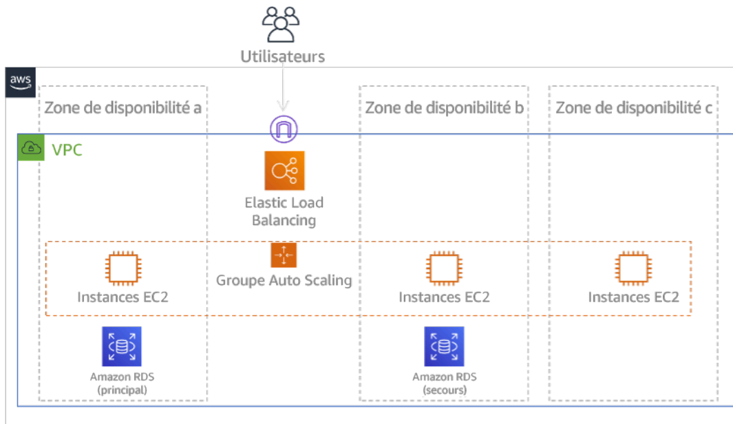
Figure 23 : architecture de multi-AZ
